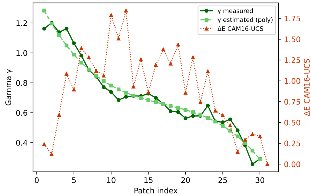
G — gamma (degree 3) mean \Delta E=0.904 std=0.490
