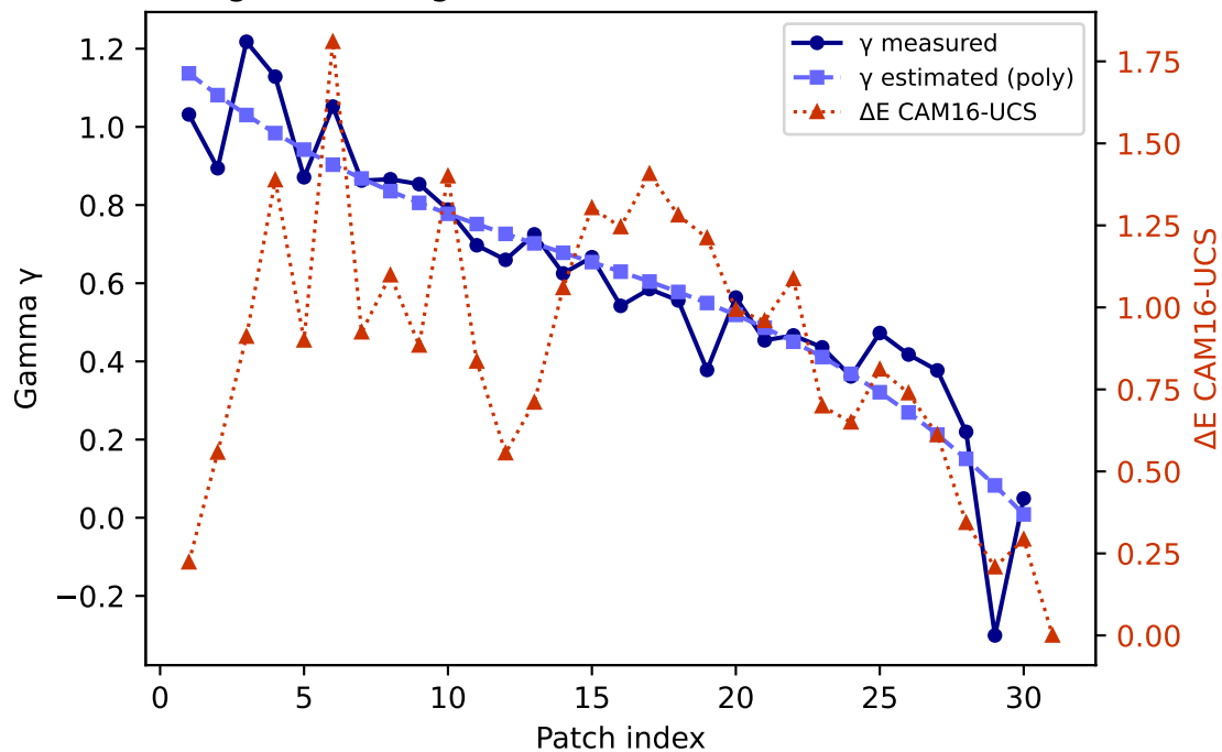
B — gamma (degree 3) mean \Delta E=0.874 std=0.406
